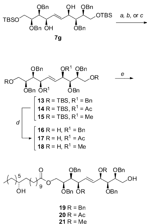
Scheme 3. Preparation of surfactant precursors 19–21 . Reaction conditions: (a) KHMDS, BnBr, THF, -78 °C \rightarrow room temp., 71%; (b) Ac 2 O, Et 3 N, DMAP, CH 2 Cl 2 , 99%; (c) KHMDS, MeI, THF, -78 °C \rightarrow room temp., 99%; (d) HOAc/H 2 O/THF (1:3:3), 50 °C, 16 : 79%, 17 : 73%, 18 : 99%; (e) ( R )-12-hydroxystearic acid, 2,4,6-trichlorobenzoyl chloride, Et 3 N, DMAP, 19 : 73%, 20 : 84%, 21 : 82%.
