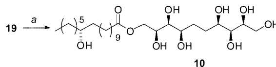
Scheme 4. Hydrogenolysis of compound 19 . Reaction conditions: (a) H 2 , Pd/C, MeOH, 61%.
