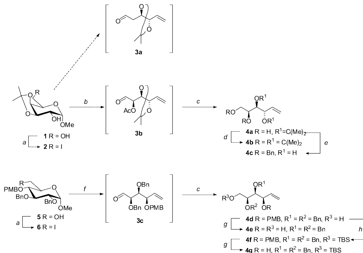
Scheme 2. Preparation of terminal olefins based on D-galactose and D-glucose. Reaction conditions: (a) \text{PPh}_3 , \text{I}_2 , imidazole, toluene, 2 : 48%, 6 : 94%; (b) i) \text{Ac}_2\text{O} , pyridine, DMAP, \text{CH}_2\text{Cl}_2 , 100%; ii) \text{Zn} , \text{NH}_4\text{Cl} , THF/ \text{H}_2\text{O} (10:1); (c) LAH, \text{Et}_2\text{O} , 4a : 55% over two steps, 4d : 71% over two steps; (d) 2-methoxypropene, p\text{TsOH} , DMF, 87%; (e) i) NaH, \text{Bu}_4\text{NI} , BnBr, THF, 61%; ii) HCl, THF, 85%; (f) \text{Zn} , \text{NH}_4\text{Cl} , THF/ \text{H}_2\text{O} (10:1); (g) DDQ, \text{CH}_2\text{Cl}_2/\text{H}_2\text{O} (25:1), 4e : 36%, 4g : 81%; (h) TBSCl, imidazole, DMF, 69%.
